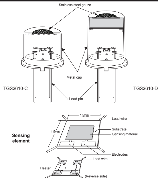
Fig. 1 - Sensor structure
