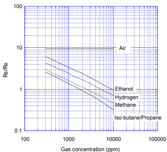
Fig. 4a - TGS2610-C00 sensitivity to various gases ( R_s/R_o )
