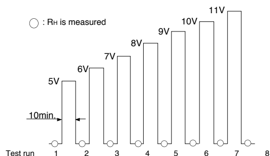
Fig. 21 - Test procedure for heater durability
