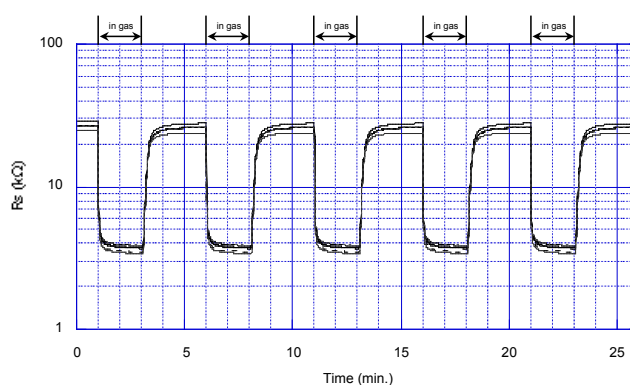
Fig. 11 - Repeatability
