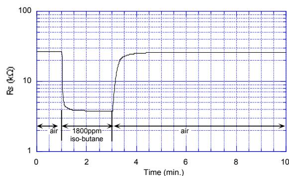
Fig. 10 - Gas response to iso-butane of TGS2610-C
