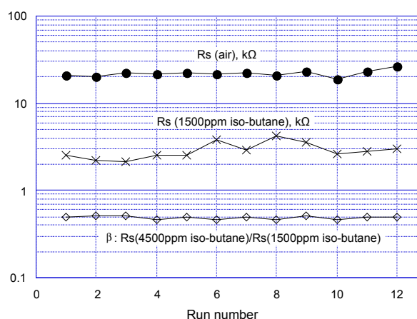
Fig. 16 - Effect of iso-butane exposure on R_s of TGS2610-C
