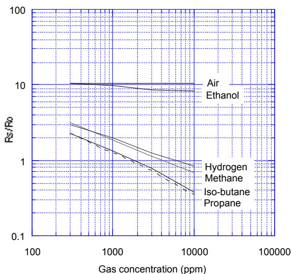
Fig. 4b - TGS2610-D00 sensitivity to various gases ( R_s/R_o )
